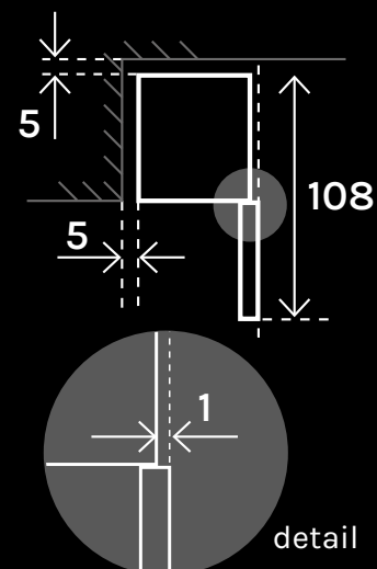
Doors opening dimensions (cm)
